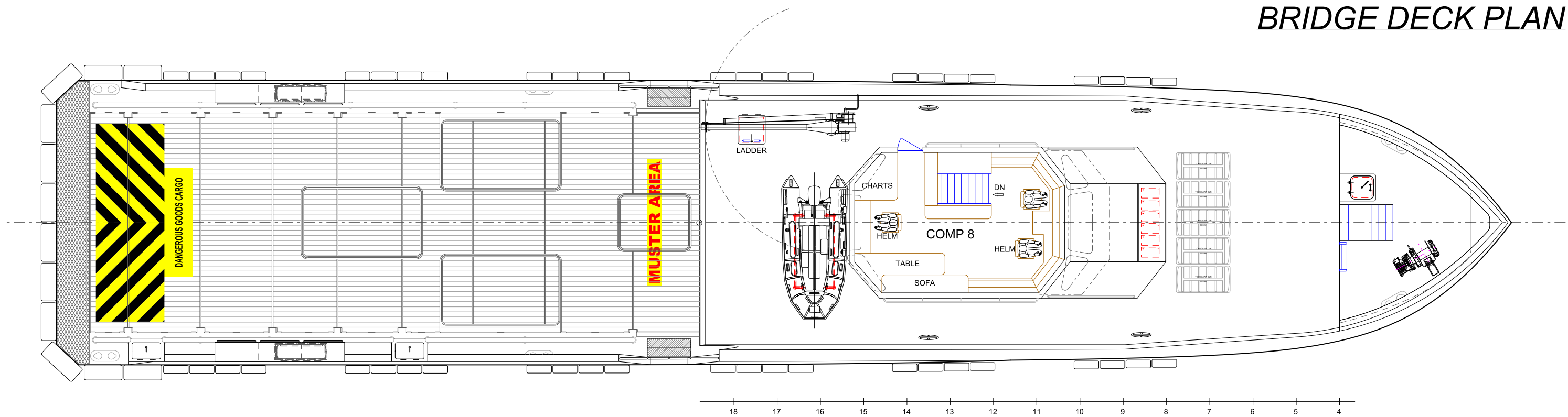
BRIDGE DECK PLAN
