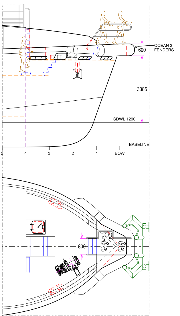
BOW BOARDING OPTION
